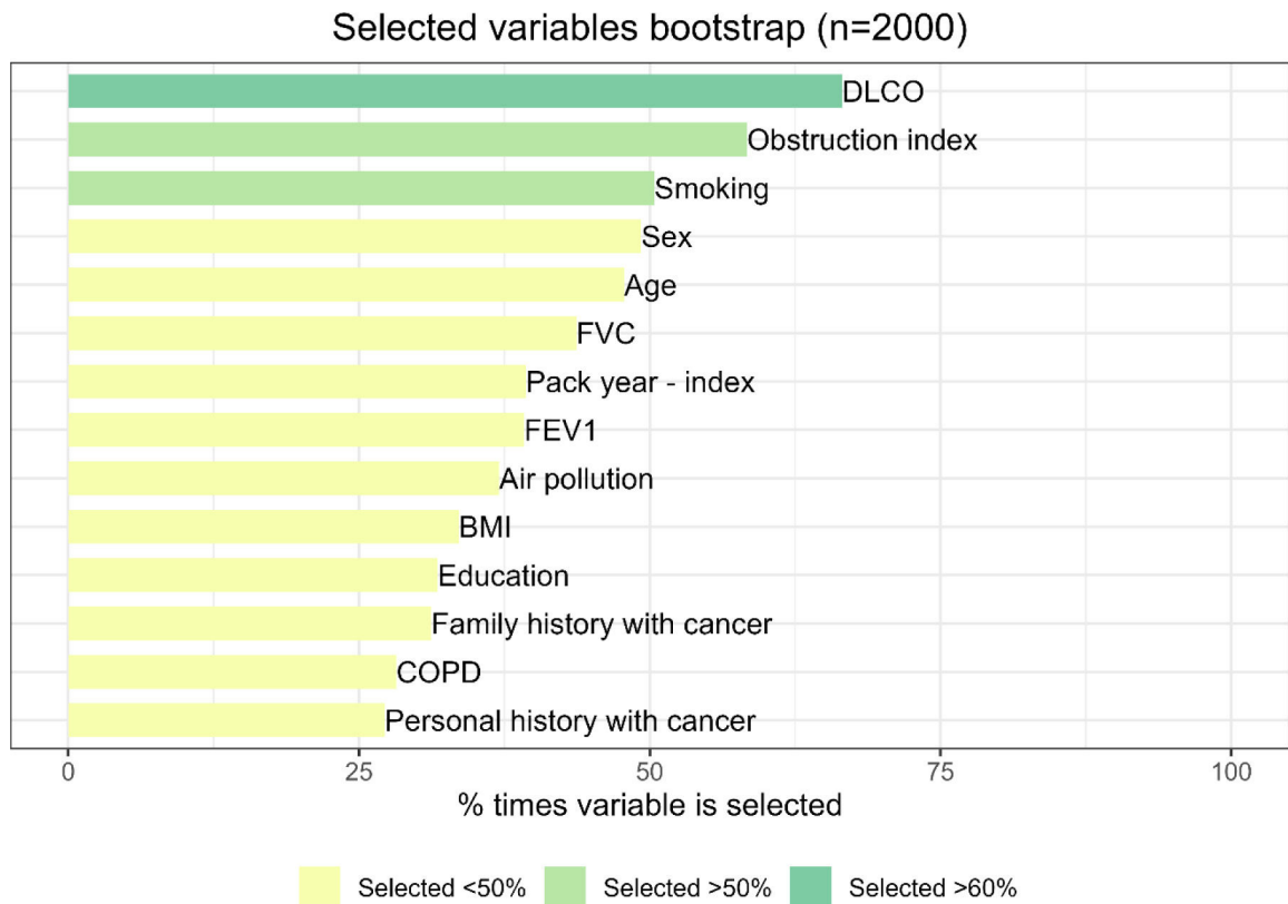
Fig. 4. Variables selected from the 2000 bootstrap model.
